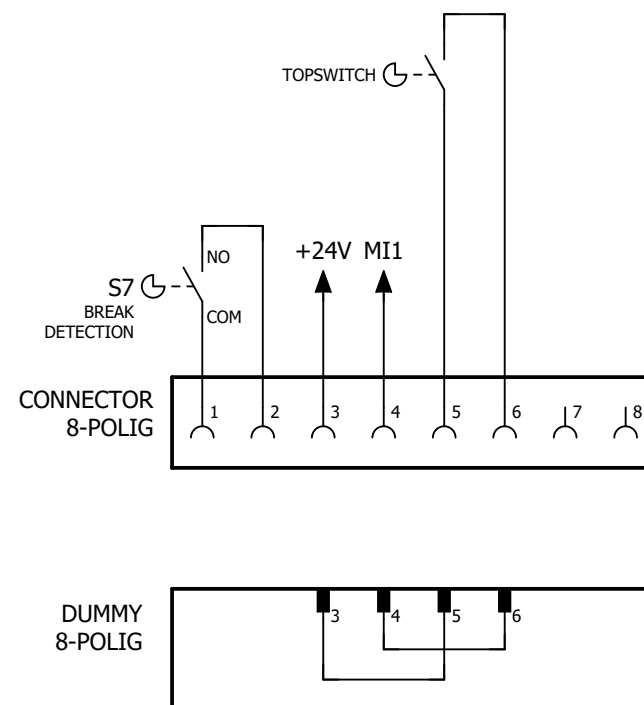
PLC - TOPSWITCH
