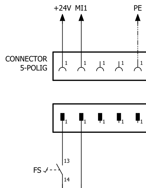
FOOT SWITCH
